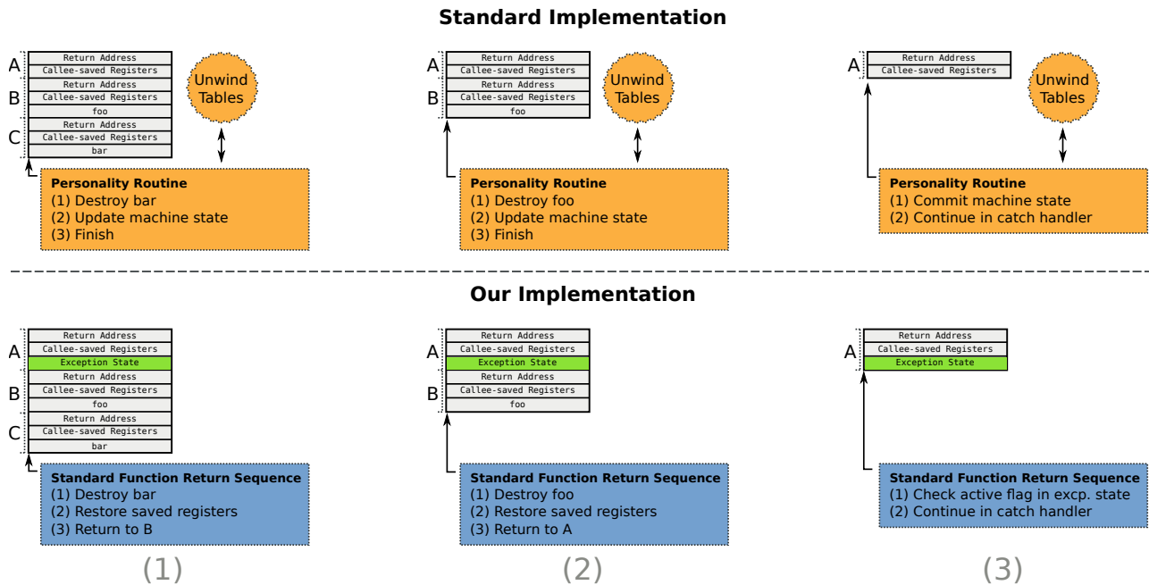
Figure 3: Stages involved in stack unwinding for the standard exception implementation (top), and our novel scheme (bottom).
