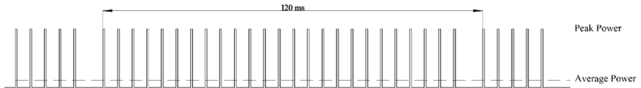
Figure 3. GSM Multiframe Showing Missing 26th Frame
