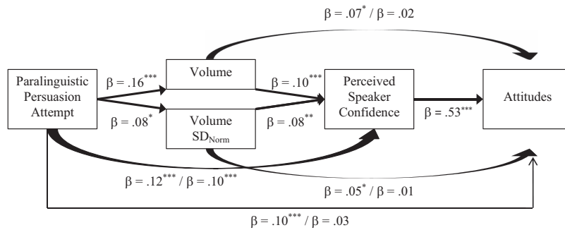
Figure 2. Lens analysis: Mediation of attitudes and confidence by speakers' vocal cues. Numbers represent standardized coefficient estimates, controlling for speaker gender (centered at zero) and its interaction with the paralinguistic persuasion attempt manipulation. Vol SD_{Norm} = Coefficient of variation for volume (Volume SD_{Norm} ). * p = .05 . ** p = .01 . *** p = .001 .
