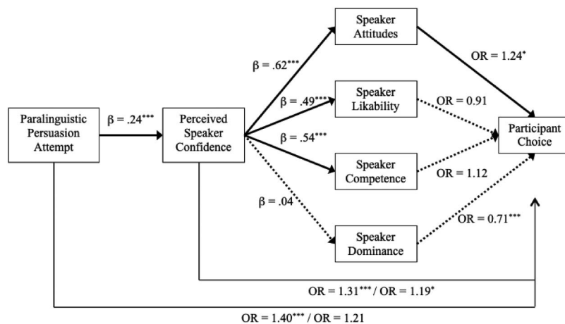
Figure 3. Experiment 4B: Mediation of choice by speakers' perceived confidence and attitudes. Numbers represent odds ratios or standardized coefficient estimates, controlling for speaker. Solid lines represent mediation pathways with significant indirect effects. *** p < .001 . * p < .05 .
